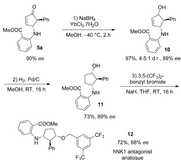
Scheme 3. Enantioselective synthesis of a cyclopentane-based hNK1 antagonist analogue.
